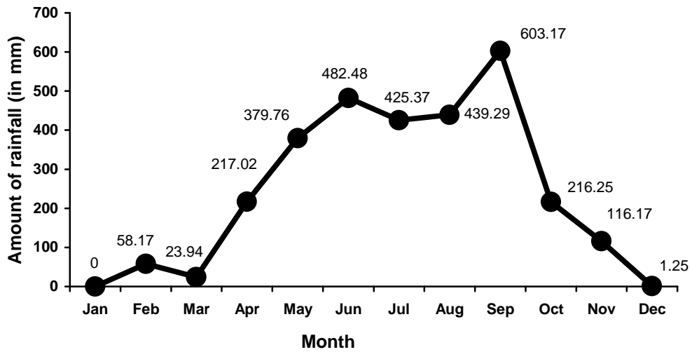
Monthly Rainfall in Mizoram -2007
