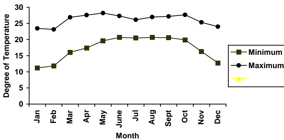
Minimum & Maximum average temperature 2007 (Aizawl City)
